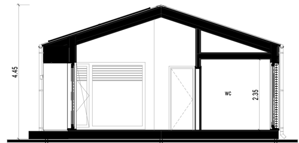
B SECTION 1:80
