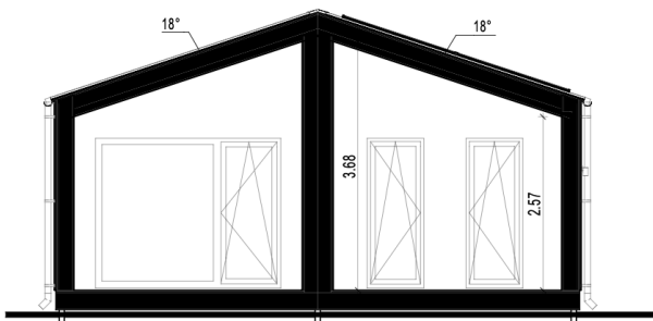
A SECTION 1:80
