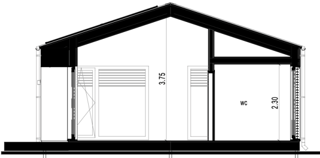
B SECTION 1:80
