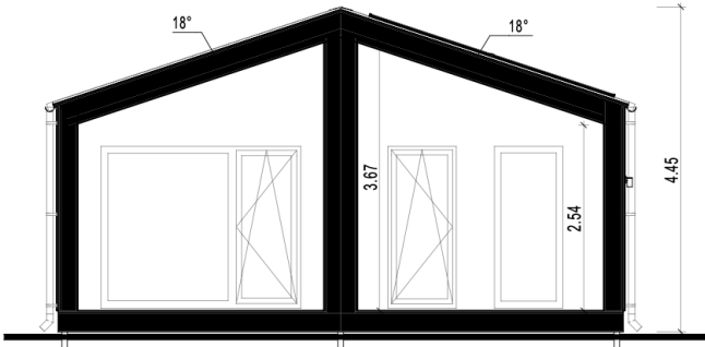
A SECTION 1:80
