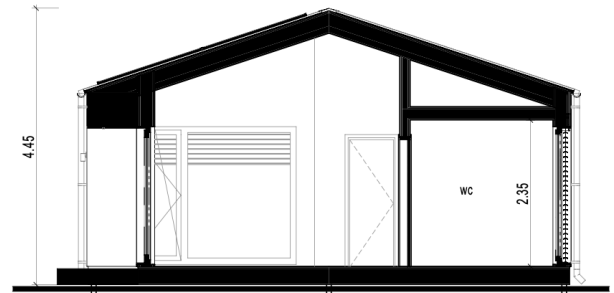
B SECTION 1:80
